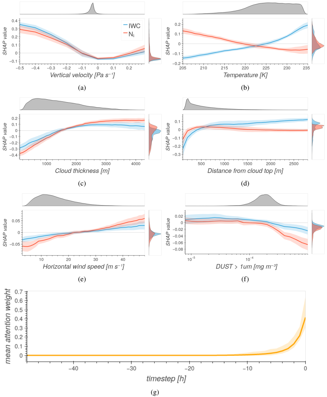
Figure 5. (a)-(f): Partial SHAP dependence plots for representative features showing the mean SHAP value per feature value for IWC in blue color and N_i in red color as solid lines. The shaded area represents the standard deviation. Additionally, the marginal distribution of the feature is displayed in grey above each plot, and the marginal SHAP value distributions are displayed on the right of each plot. Note that the absolute SHAP values of IWC and N_i are not directly comparable as the SHAP value indicates the contribution of a feature to the prediction value, and the two variables have different yet similar distributions. The plots show only feature values with at least 5000 occurrences in the test data set. (g): Mean of attention weight per timestep. Attention weights are learned during the training process of the LSTM model and represent the relative importance of the input data per timestep. .
